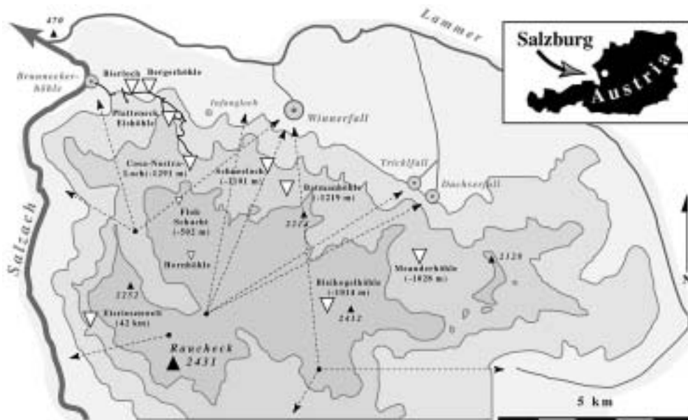
Fig. 1. Topographic map of the Tennengebirge (contour interval 500 m). Dashed lines correspond to water tracing.
