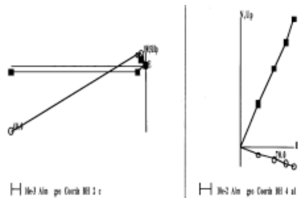
Fig. 8. Orthogonal Zijdeveld plots showing the NRM vector evolution during AF demagnetization up to 100 mT (BH 2, BH 4 samples).
