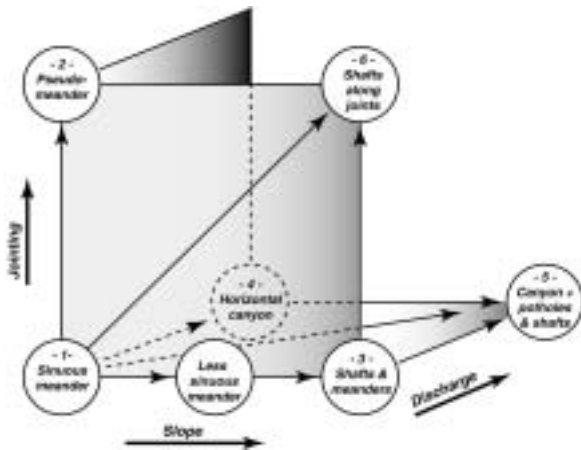
Fig. 9. Predominant conduits in the vadose zone, in relation to slope, jointing, and discharge.
