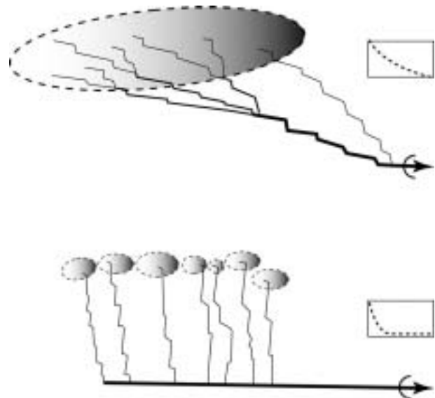
Fig. 10. Morphology of passage in relation to jointing intensity. Above, with little jointing, profile is slightly concave and strongly hierarchical (e.g. Vercors). Below, in highly jointed rock, profile is strongly concave and only slightly hierarchical (e.g. Tennenbergeirge).
