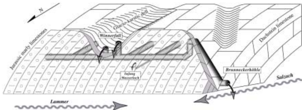
Fig. 11. Impermeable Jurassic strata dam the Dachstein Limestone aquifer (not to scale). Spring outlets are located at structural lows where glaciers have eroded the Jurassic beds.
