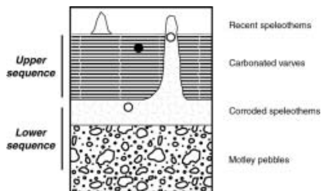
Fig. 7. Generalized stratigraphic section of the sediments in the Bergerhöhle and Bierloch system. Black circles = normal paleomagnetic orientation; white circles = reversed paleomagnetism.
