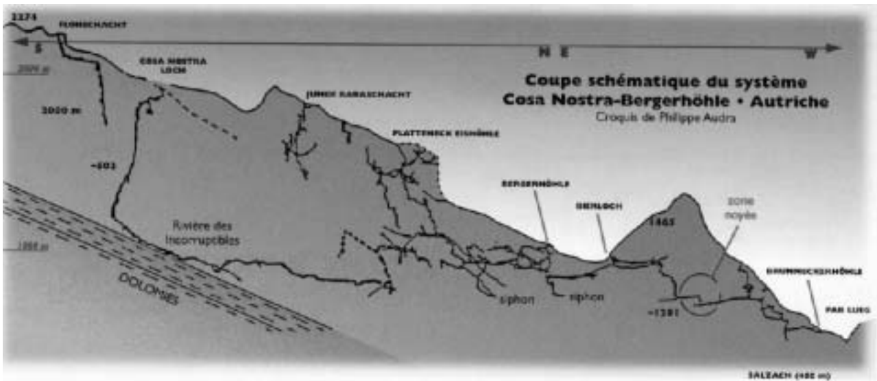
Fig. 5. Cross section of the Cosa Nostra - Bergerhöhle System.
