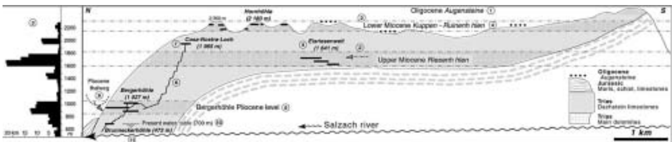
Fig. 2. The Cosa Nostra - Bergerhöhle system and the Tennengebirge (see also text). To the left (3), relationship between cave passages altitude and old karst levels (after Klappacher & Knapczyk 1985). Karst development began during the Oligocene beneath Augensteine (1). During the Miocene, horizontal systems developed with alpine water inputs (2), showing different levels (3) related to successive phases of stability: Ruinenhöhlen (4) and Riesenhöhlen (e.g. Eisriesenwelt - 5). Following Pliocene uplift, alpine systems developed (e.g. Cosa Nostra – Bergerhöhle - 6). Entrance horizontal tubes correspond to a Miocene level (7). Shaft series (6) connect to horizontal tubes from Bergerhöhle-Bierloch (8), corresponding to Pliocene base level (9). Present water-table at -700 m (10) pours into Brunnecker Cave, which connects to Salzach base level (11).
