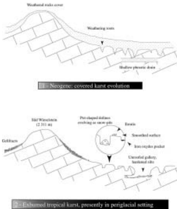
Fig. 3. Diagram showing the evolution of the Windischriedel karst, from the Late Tertiary (top) to the Pleistocene (bottom).
