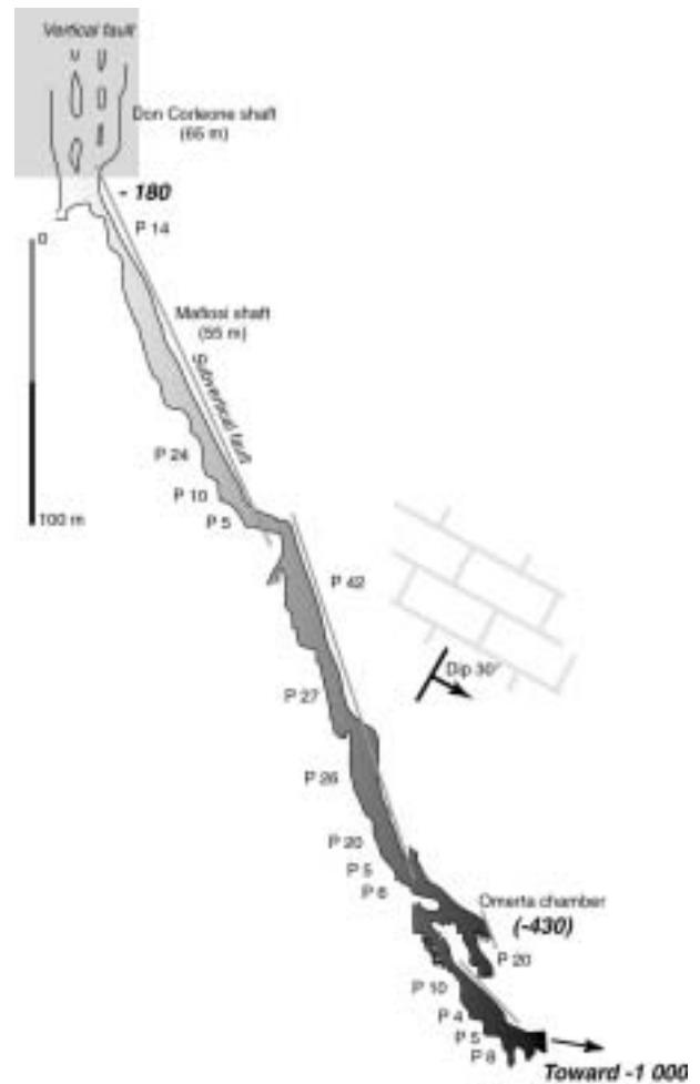
Fig. 6. Profile showing “Stairs beneath a faulted roof” of Cosa-Nostra Loch, a predominant aspect of vertical systems.
